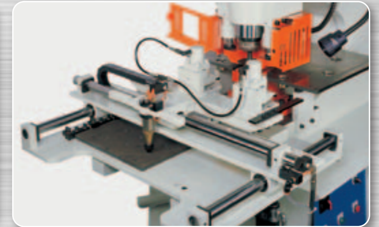
*Optional duplicating table with hydraulic stripper and hydraulic clamping for fast and accurate repetition work. (S/SD/KD and PM models only)
