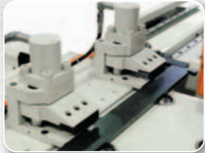
Operate in semi-automatic mode with use of gauging piece allows punching holes near the edge of the material.
